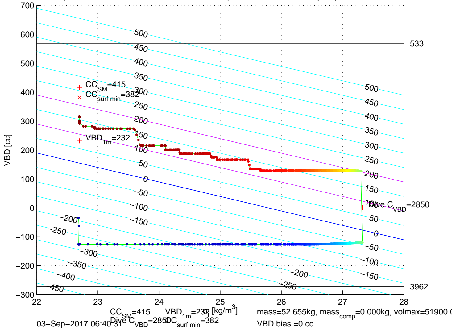
p6350338: SG635 Mission 7 Jul 2017 03-Sep-2017 06:25:03Z – buoyancy contoured
