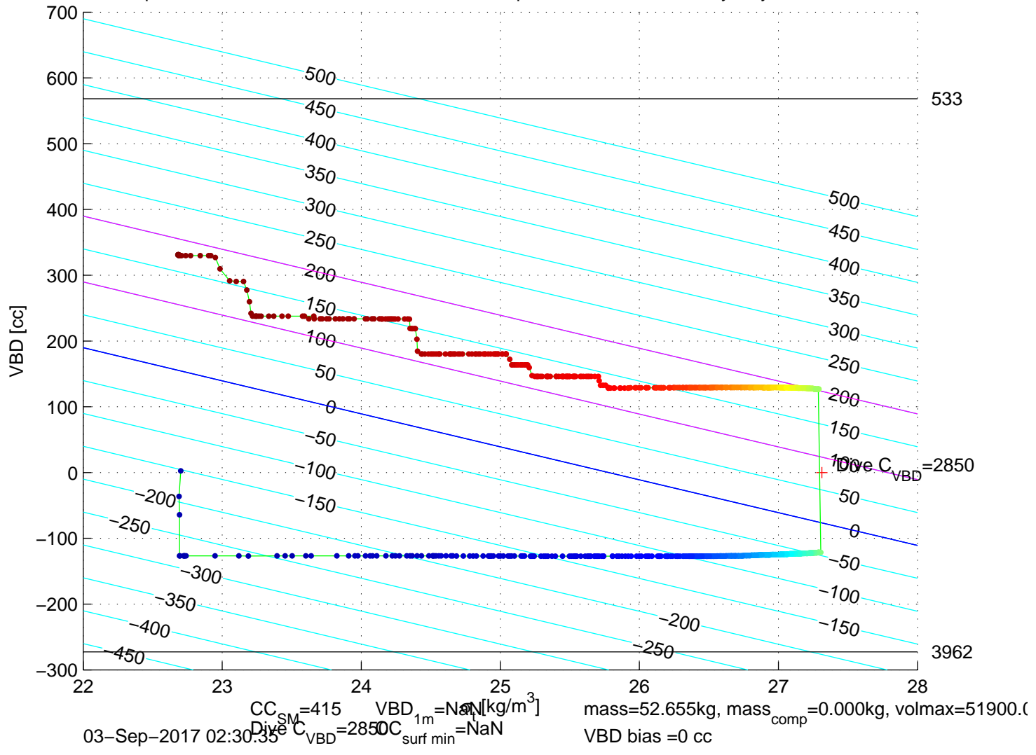
p6350337: SG635 Mission 7 Jul 2017 03-Sep-2017 02:13:00Z – buoyancy contoured
