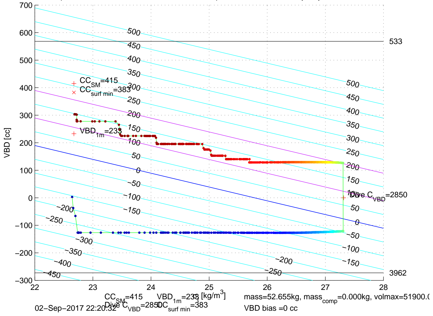
p6350336: SG635 Mission 7 Jul 2017 02-Sep-2017 22:03:34Z – buoyancy contoured
