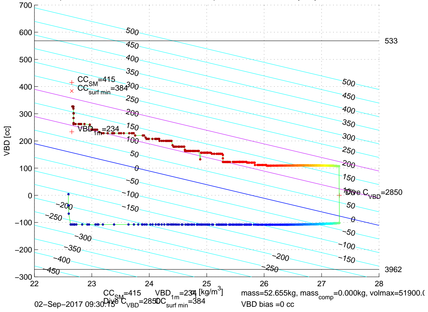
p6350333: SG635 Mission 7 Jul 2017 02-Sep-2017 09:02:16Z – buoyancy contoured
