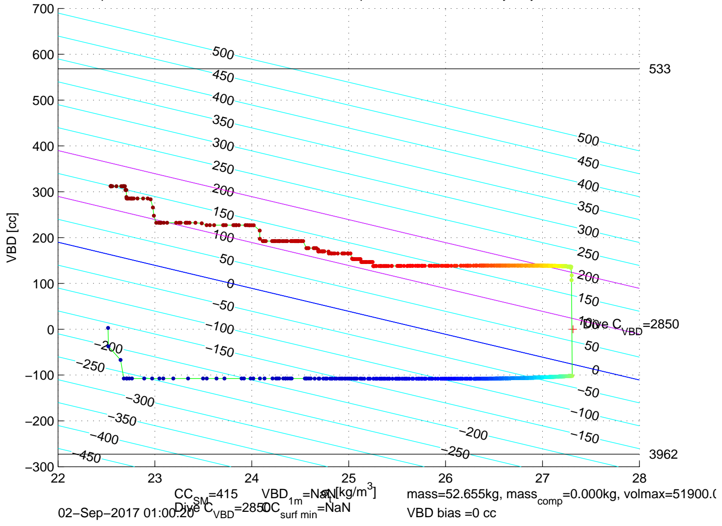
p6350331: SG635 Mission 7 Jul 2017 02-Sep-2017 00:39:08Z – buoyancy contoured
