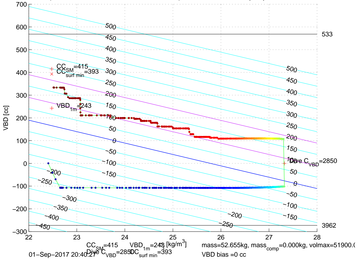
p6350330: SG635 Mission 7 Jul 2017 01-Sep-2017 20:17:01Z – buoyancy contoured
