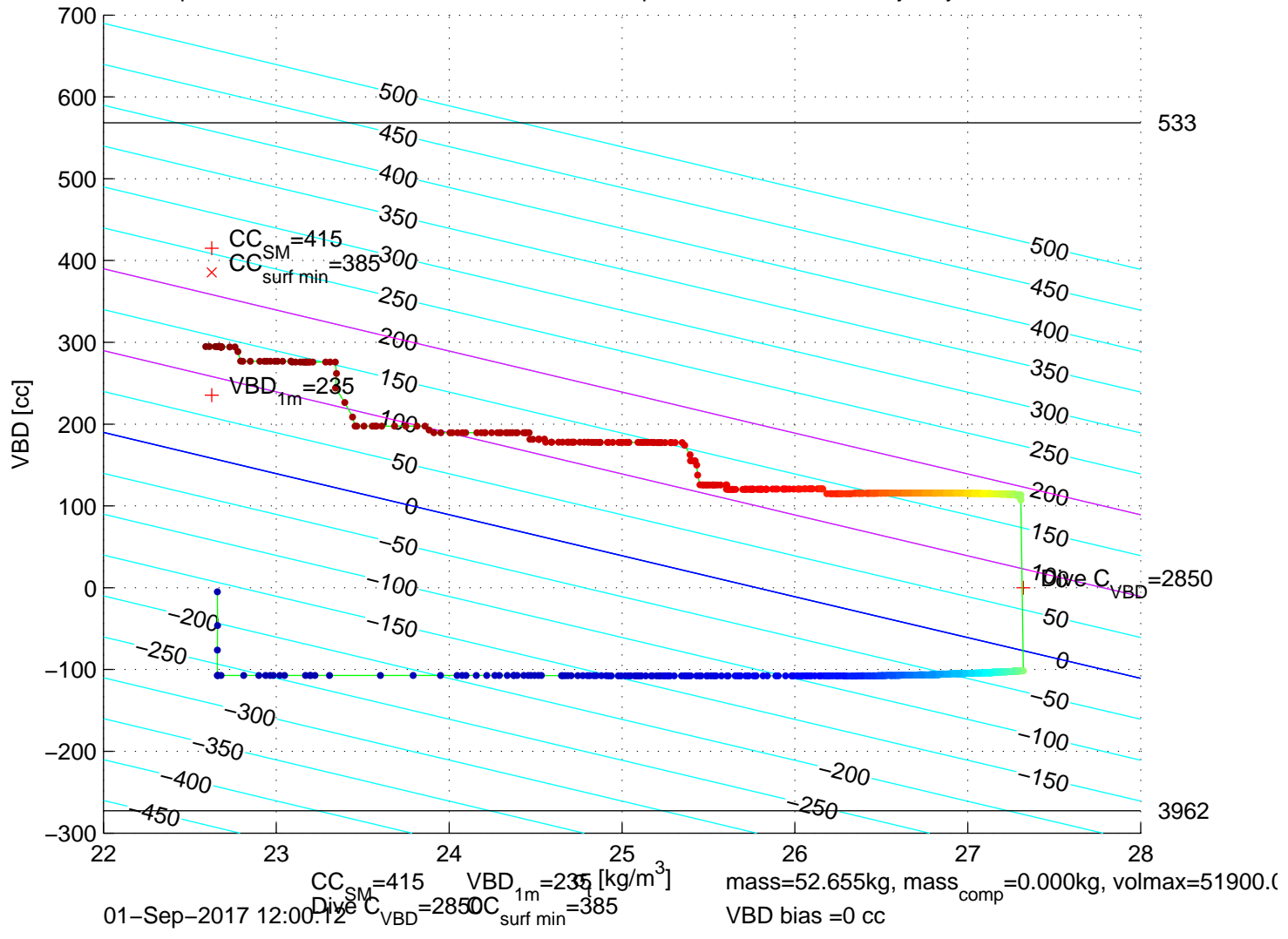
p6350328: SG635 Mission 7 Jul 2017 01-Sep-2017 11:26:41Z – buoyancy contoured
