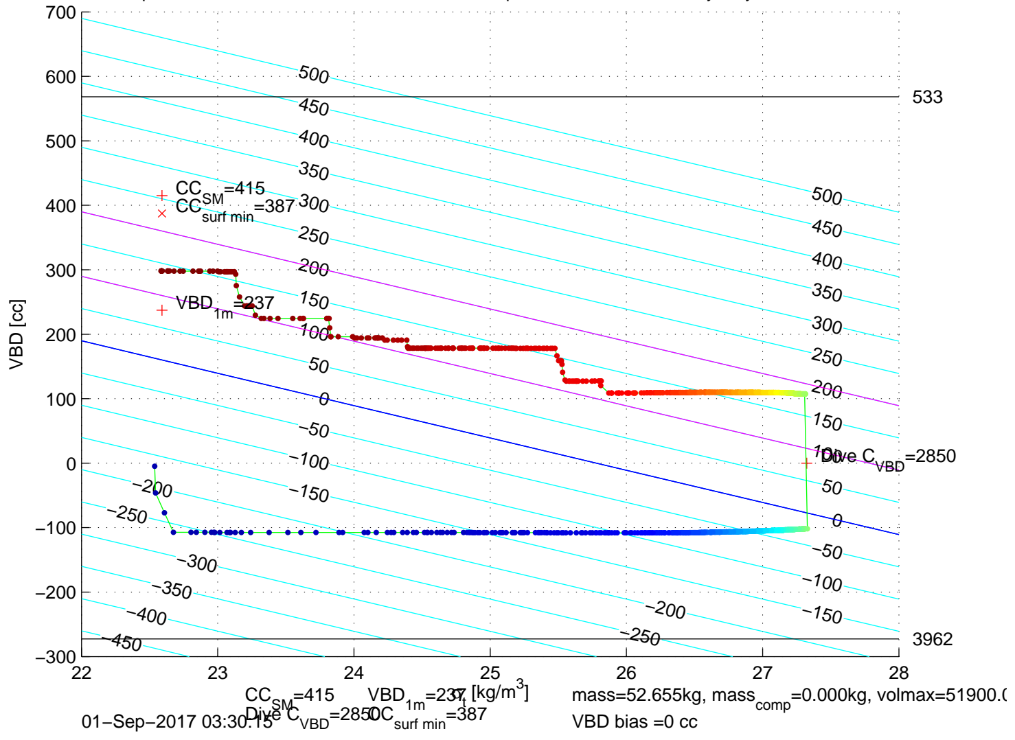
p6350326: SG635 Mission 7 Jul 2017 01-Sep-2017 03:03:46Z – buoyancy contoured
