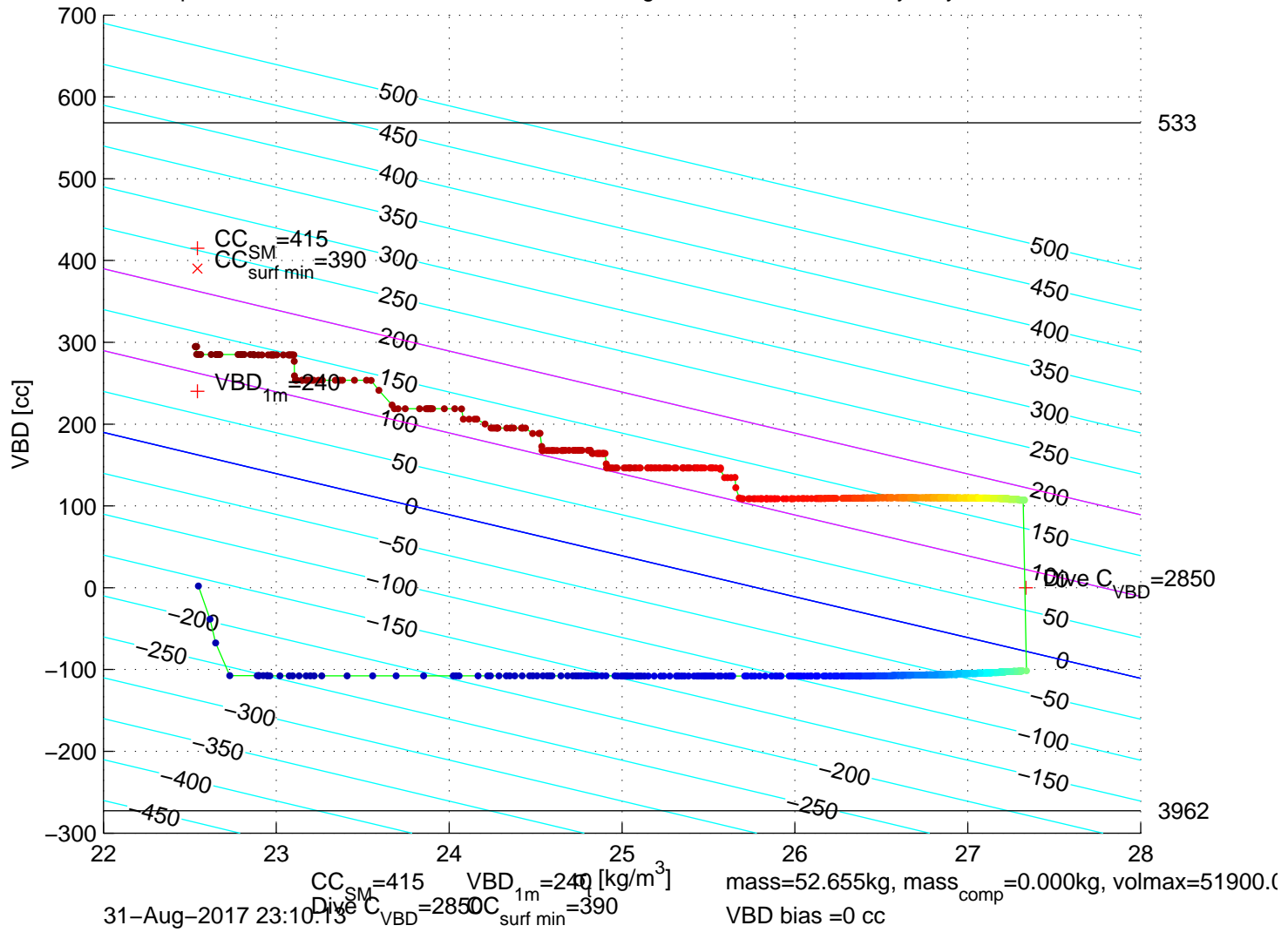
p6350325: SG635 Mission 7 Jul 2017 31-Aug-2017 22:41:41Z – buoyancy contoured
