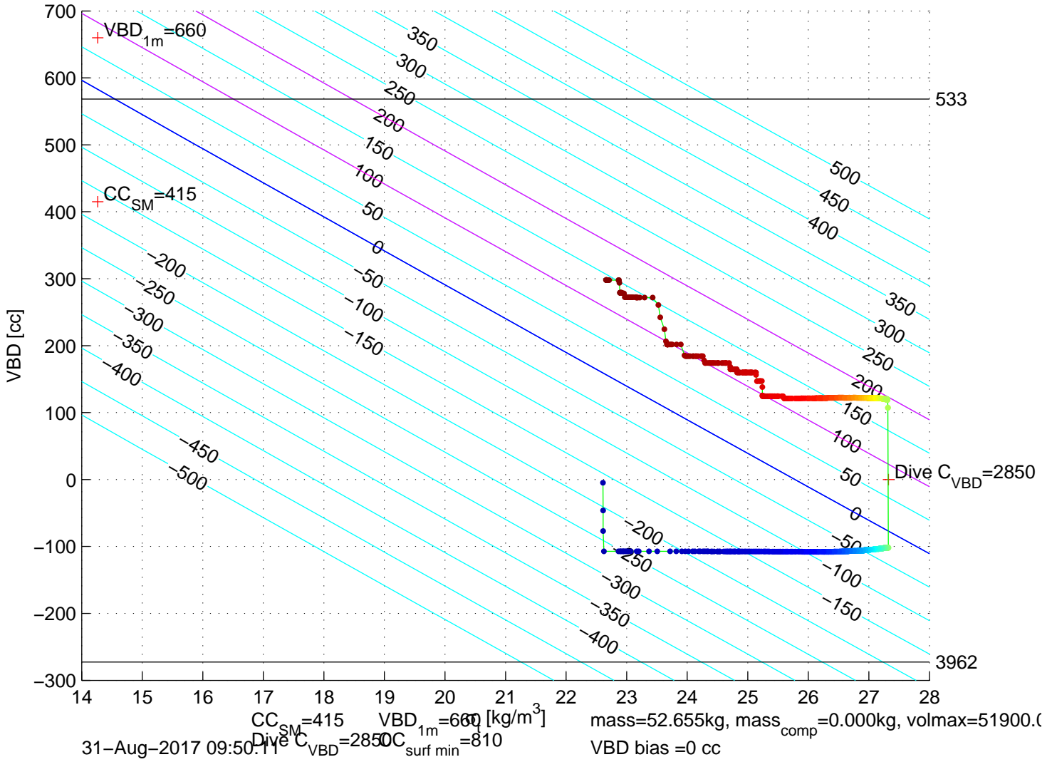
p6350322: SG635 Mission 7 Jul 2017 31-Aug-2017 09:31:52Z - buoyancy contoured
