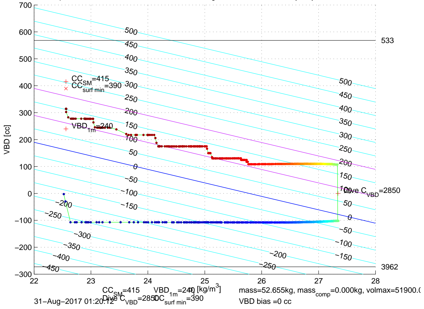
p6350320: SG635 Mission 7 Jul 2017 31-Aug-2017 00:49:40Z – buoyancy contoured
