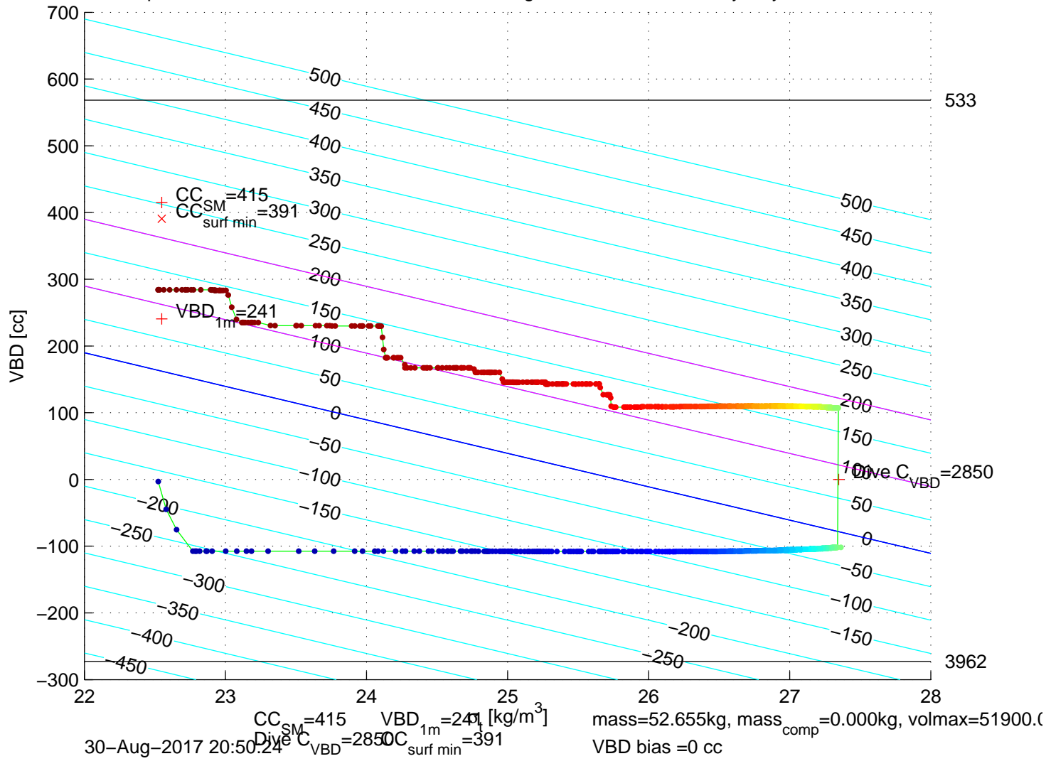
p6350319: SG635 Mission 7 Jul 2017 30-Aug-2017 20:26:37Z – buoyancy contoured
