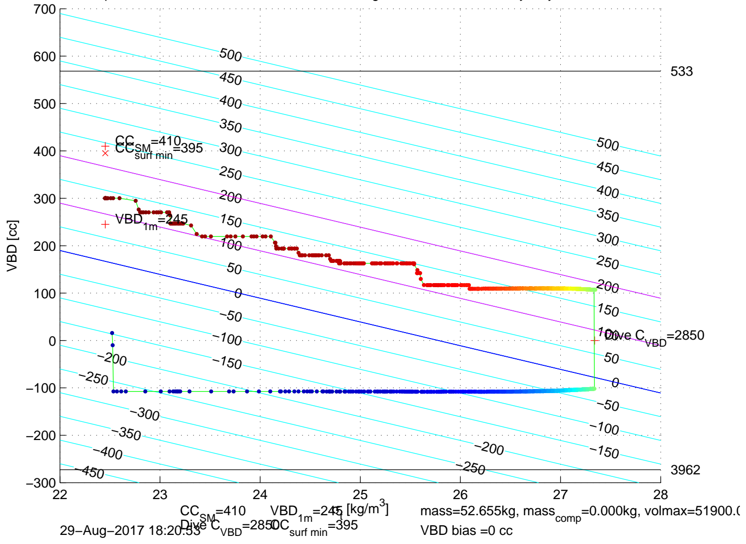
p6350313: SG635 Mission 7 Jul 2017 29-Aug-2017 17:56:37Z – buoyancy contoured
