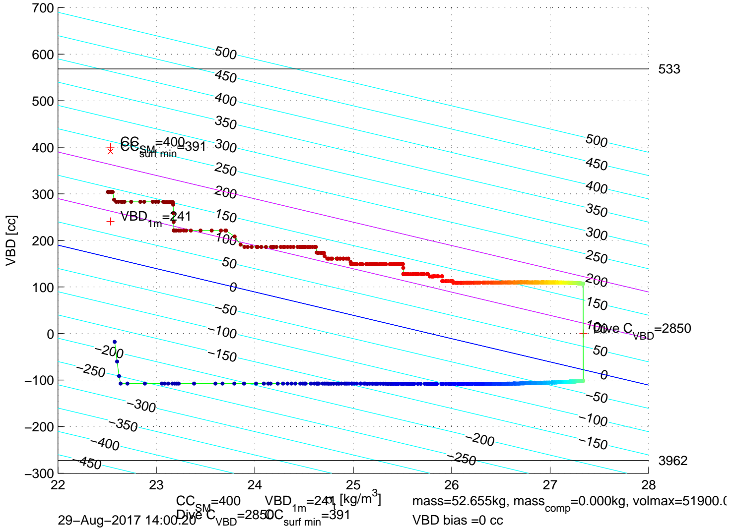
p6350312: SG635 Mission 7 Jul 2017 29-Aug-2017 13:24:39Z – buoyancy contoured
