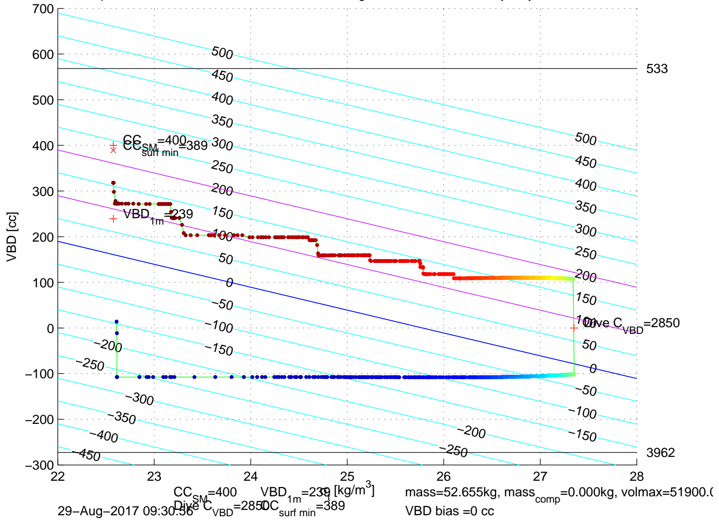
p6350311: SG635 Mission 7 Jul 2017 29-Aug-2017 08:53:19Z – buoyancy contoured
