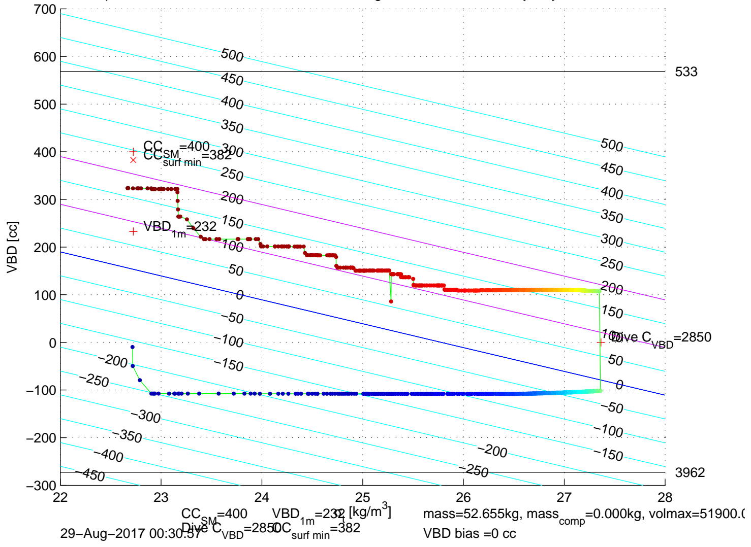
p6350309: SG635 Mission 7 Jul 2017 28-Aug-2017 23:51:33Z – buoyancy contoured
