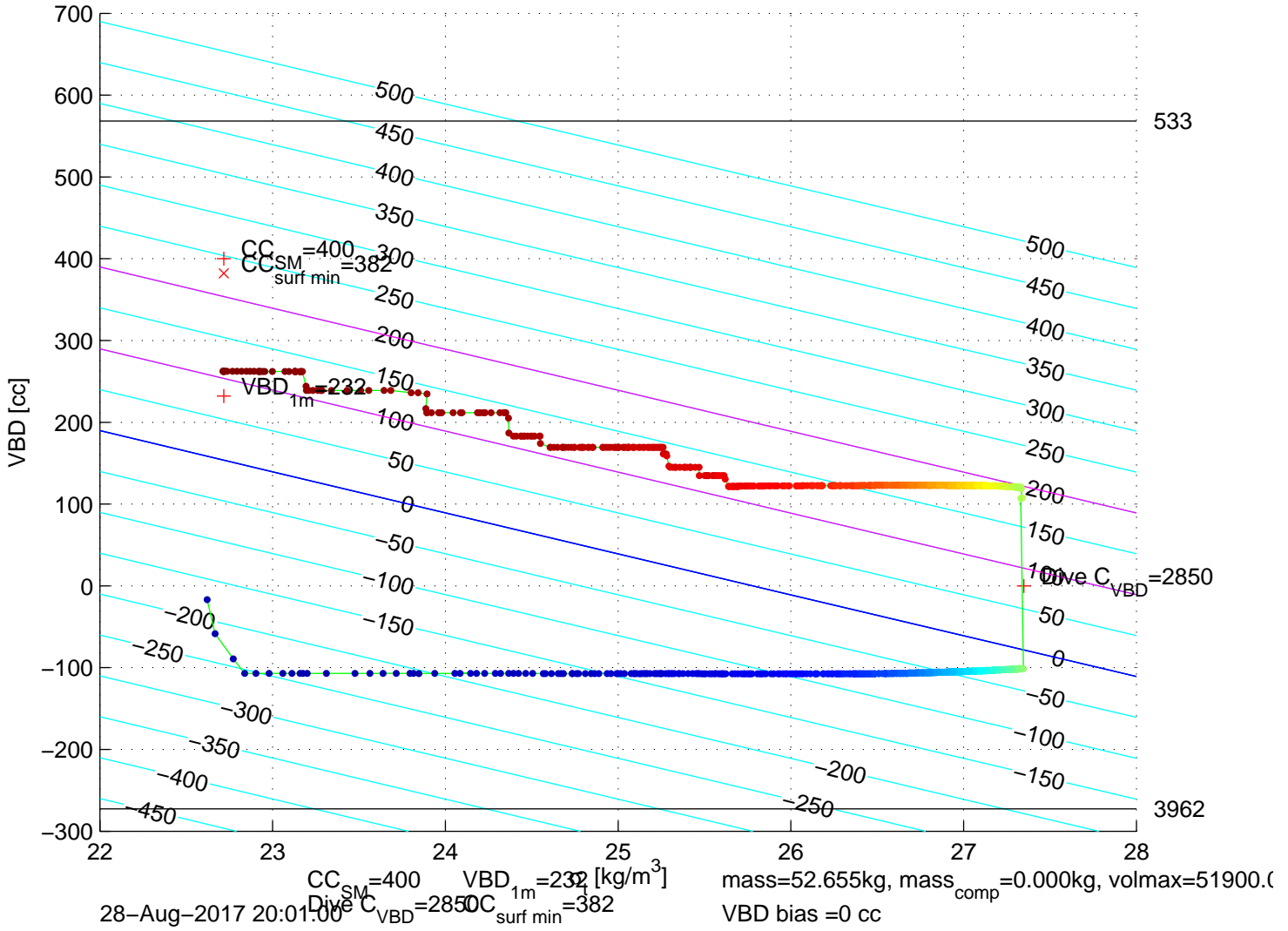
p6350308: SG635 Mission 7 Jul 2017 28-Aug-2017 19:29:53Z – buoyancy contoured
