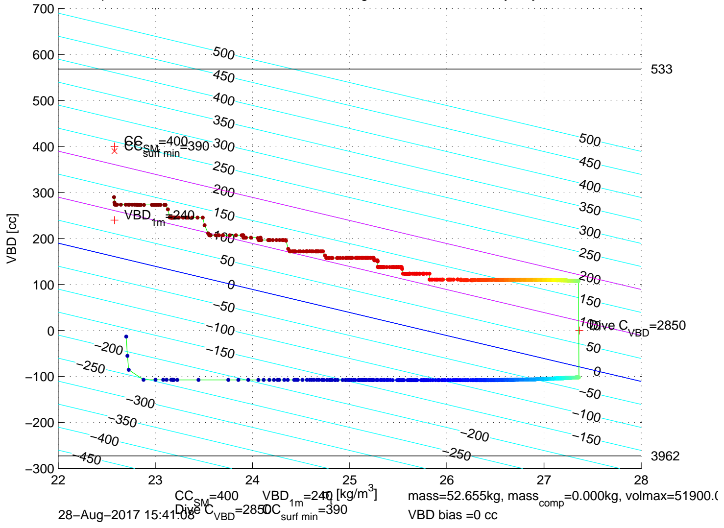
p6350307: SG635 Mission 7 Jul 2017 28-Aug-2017 15:00:02Z – buoyancy contoured
