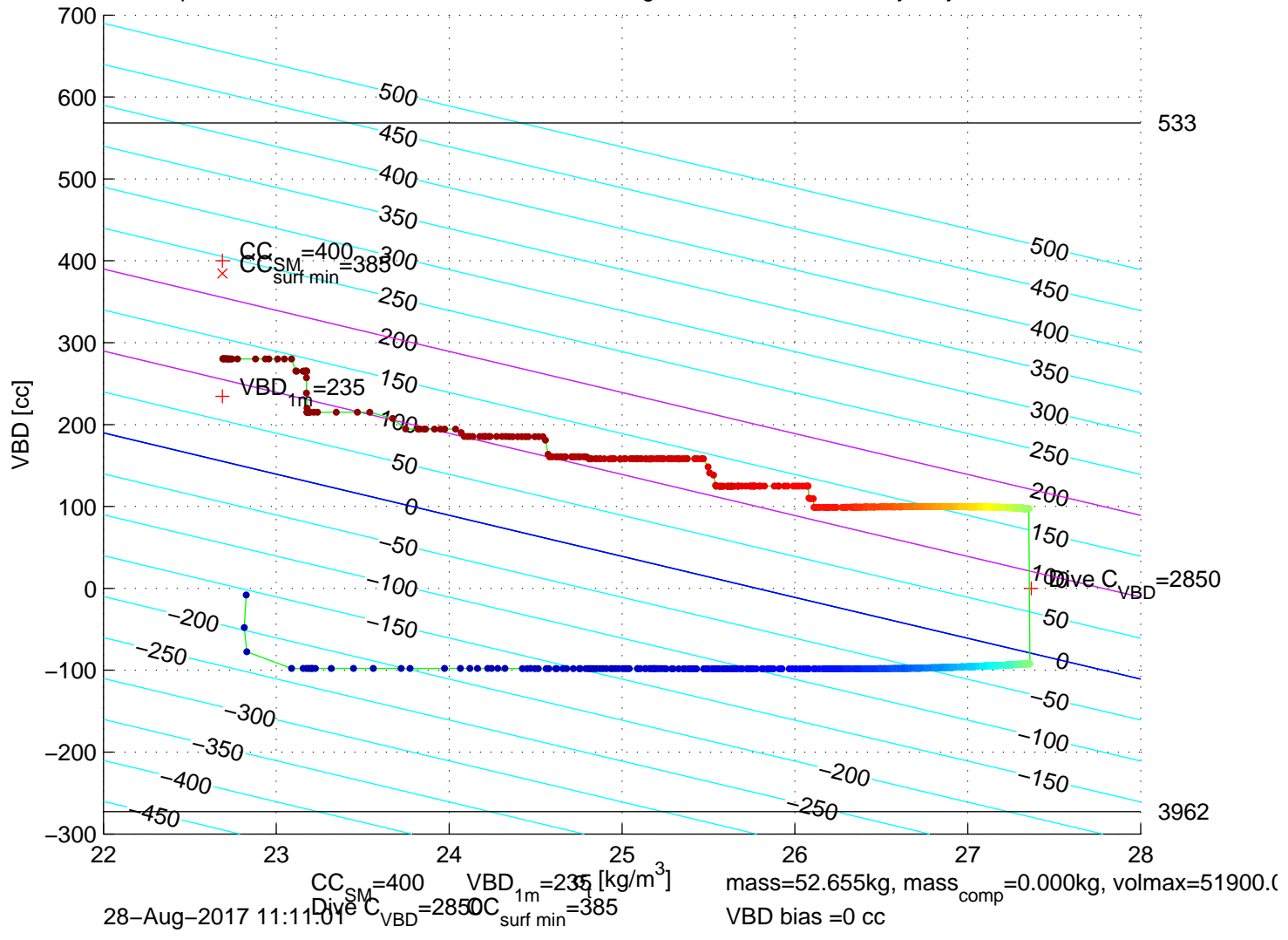
p6350306: SG635 Mission 7 Jul 2017 28-Aug-2017 10:24:26Z – buoyancy contoured
