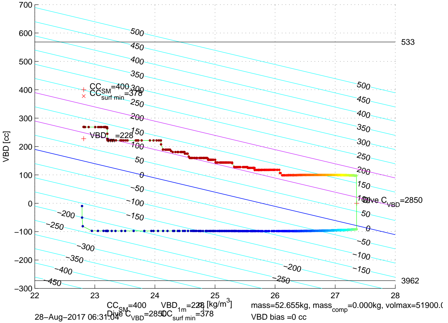
p6350305: SG635 Mission 7 Jul 2017 28-Aug-2017 05:47:03Z – buoyancy contoured
