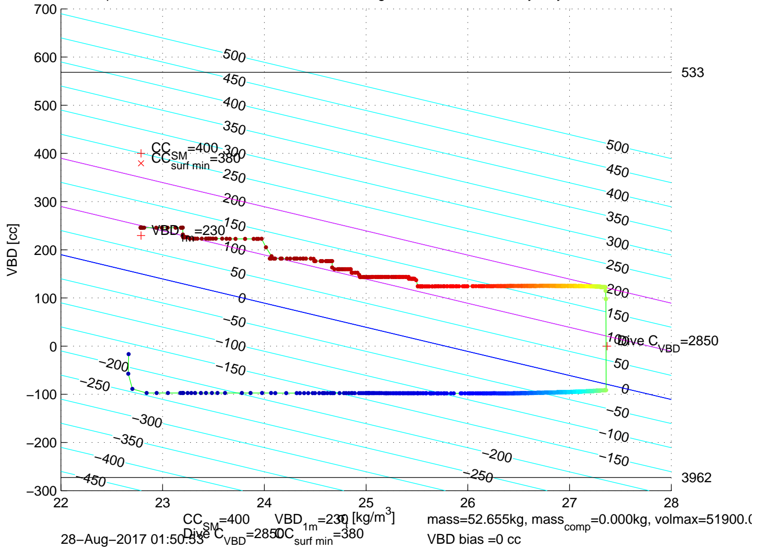
p6350304: SG635 Mission 7 Jul 2017 28-Aug-2017 01:25:26Z – buoyancy contoured
