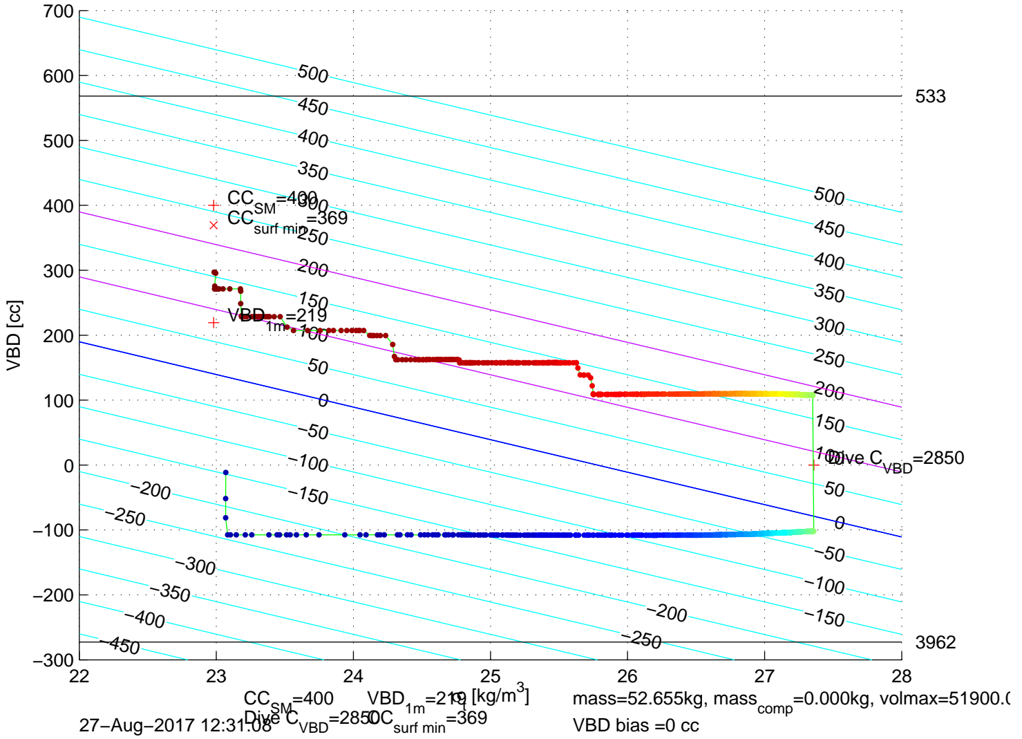
p6350301: SG635 Mission 7 Jul 2017 27-Aug-2017 11:46:15Z – buoyancy contoured
