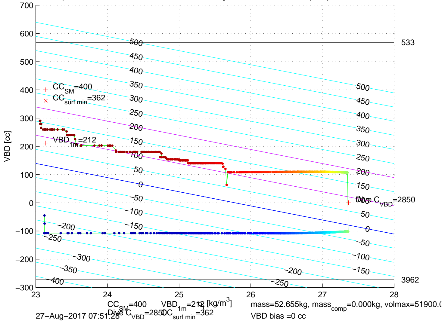
p6350300: SG635 Mission 7 Jul 2017 27-Aug-2017 07:18:32Z – buoyancy contoured
