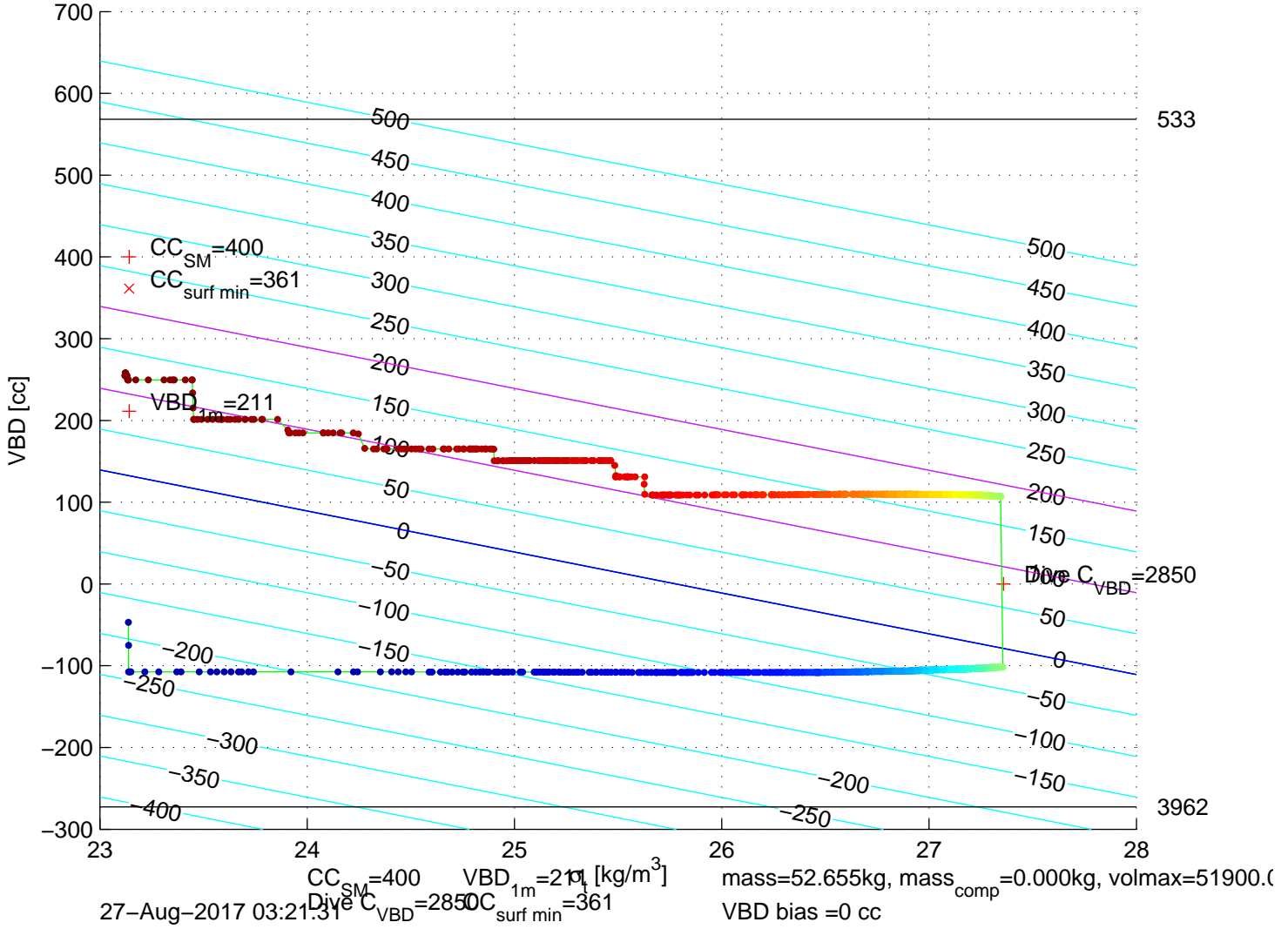
p6350299: SG635 Mission 7 Jul 2017 27-Aug-2017 02:51:14Z – buoyancy contoured
