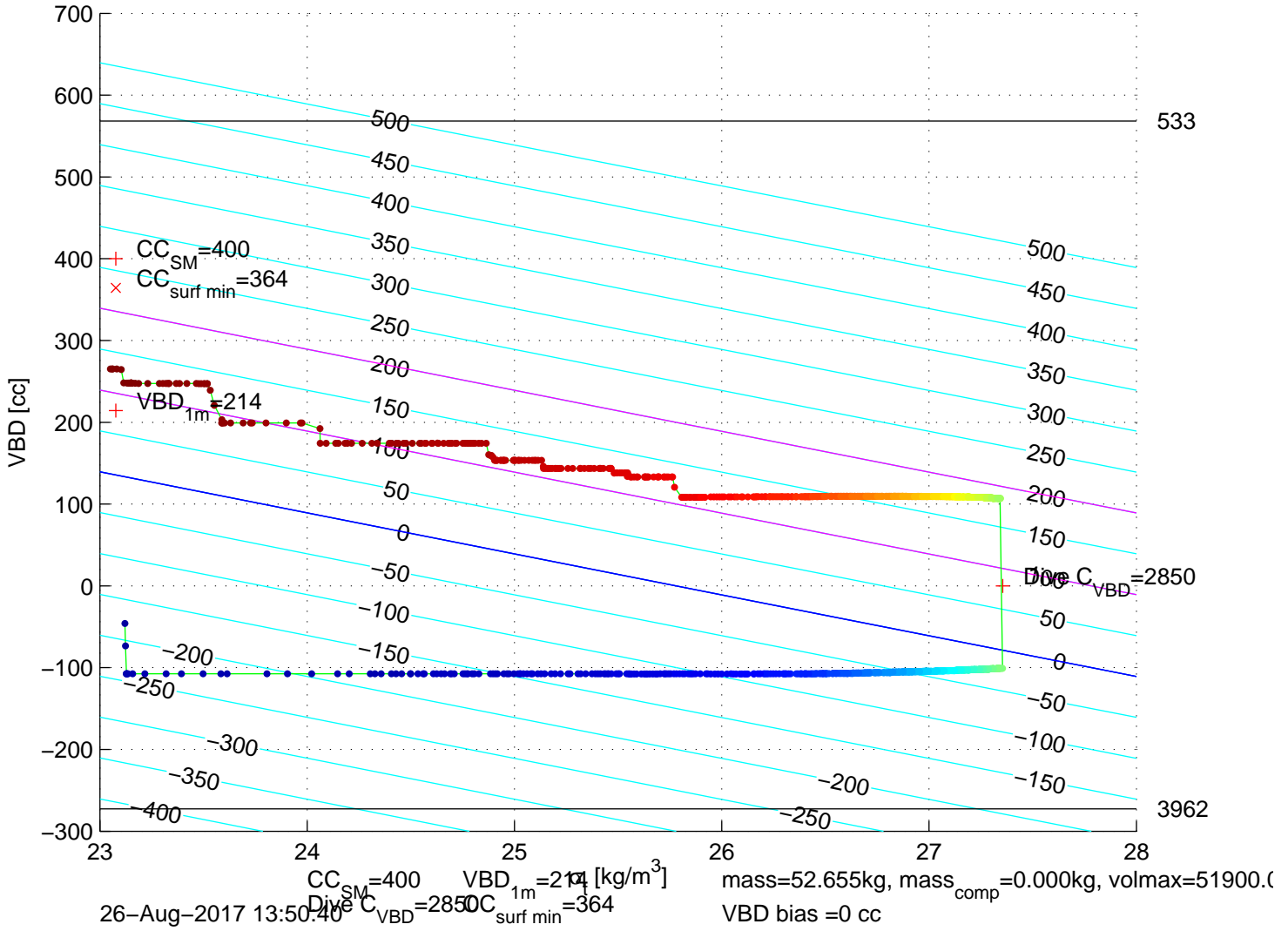
p6350296: SG635 Mission 7 Jul 2017 26-Aug-2017 13:15:44Z – buoyancy contoured
