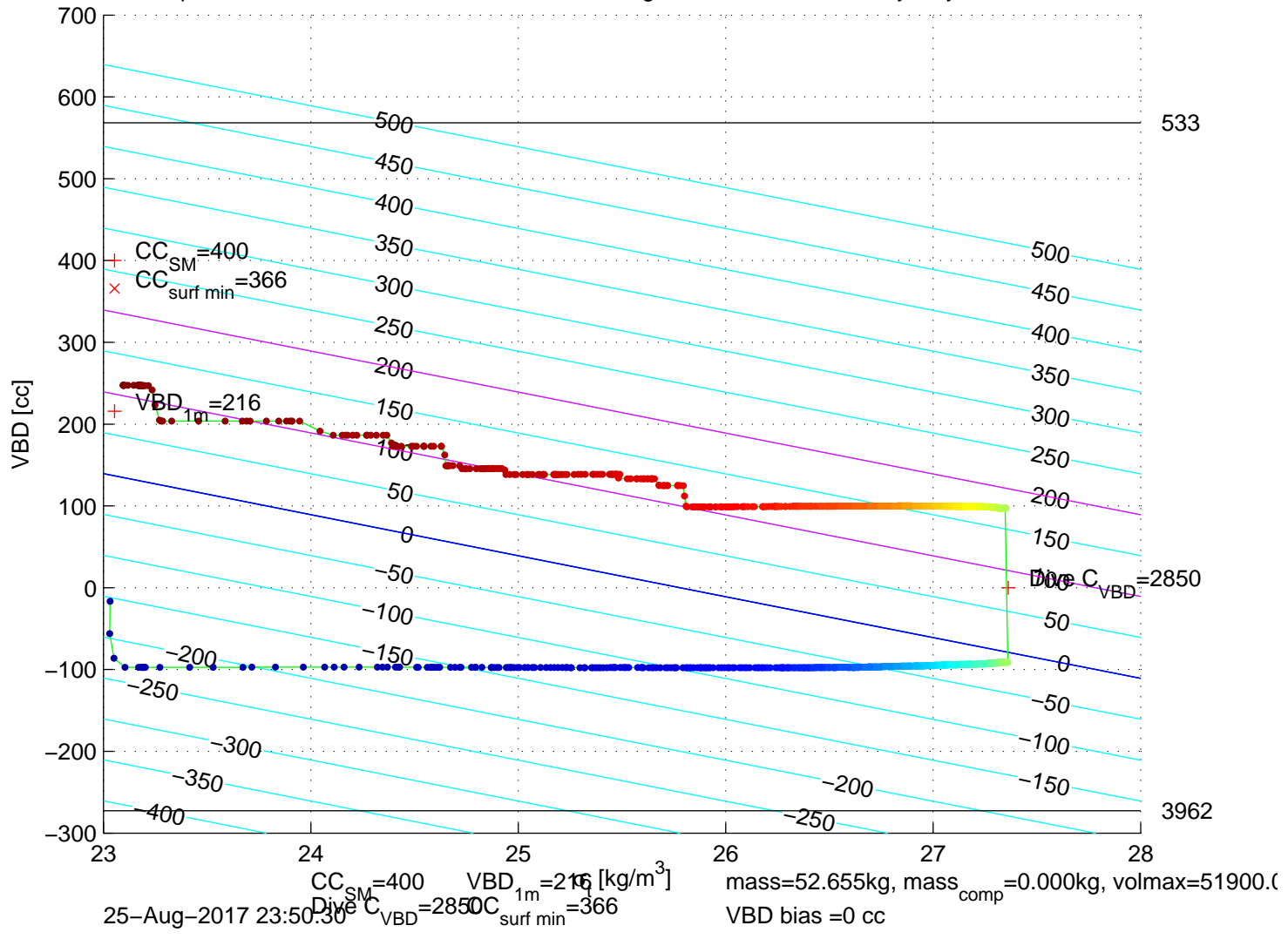
p6350293: SG635 Mission 7 Jul 2017 25-Aug-2017 23:00:39Z – buoyancy contoured
