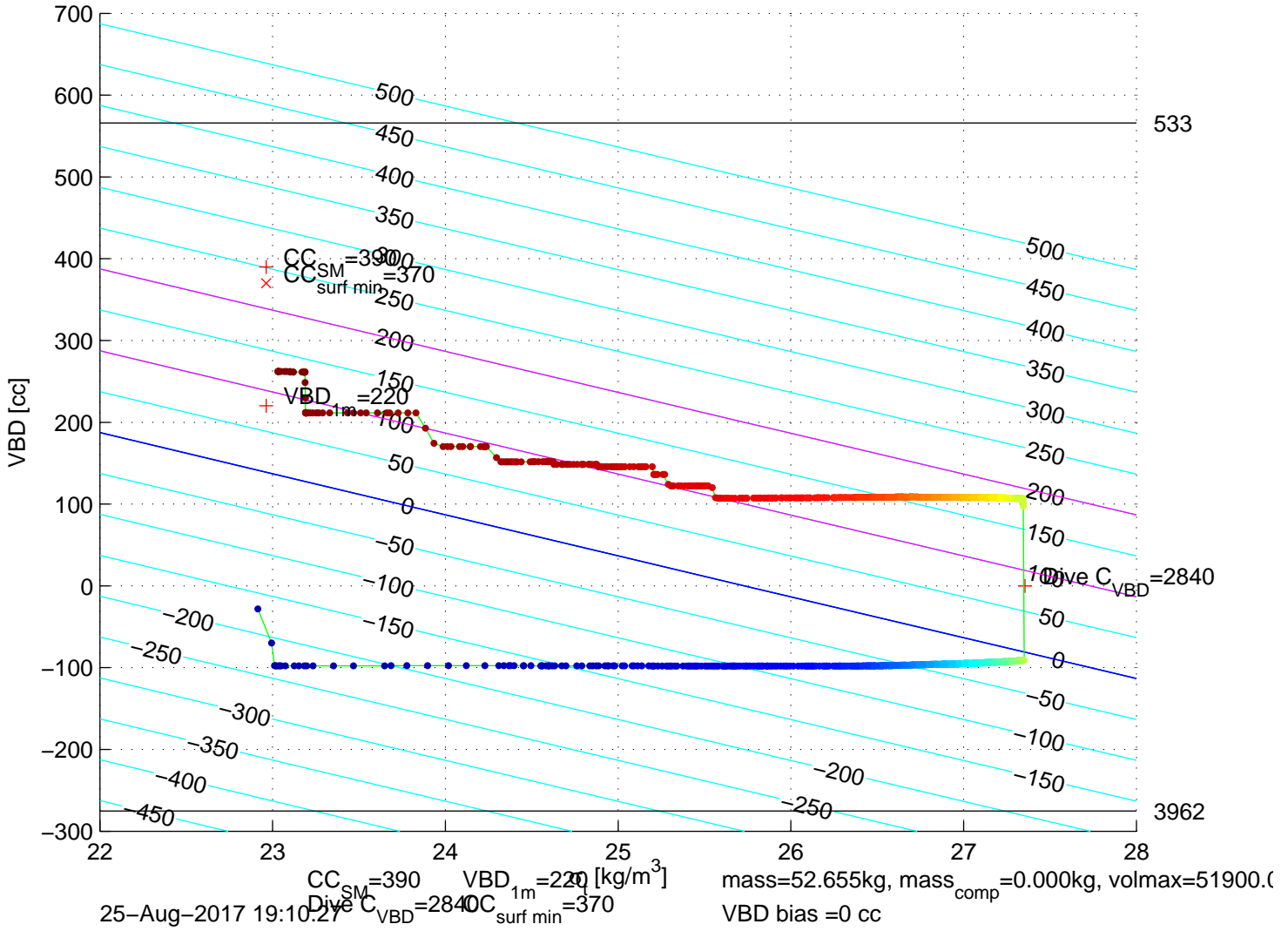
p6350292: SG635 Mission 7 Jul 2017 25-Aug-2017 18:23:53Z – buoyancy contoured
