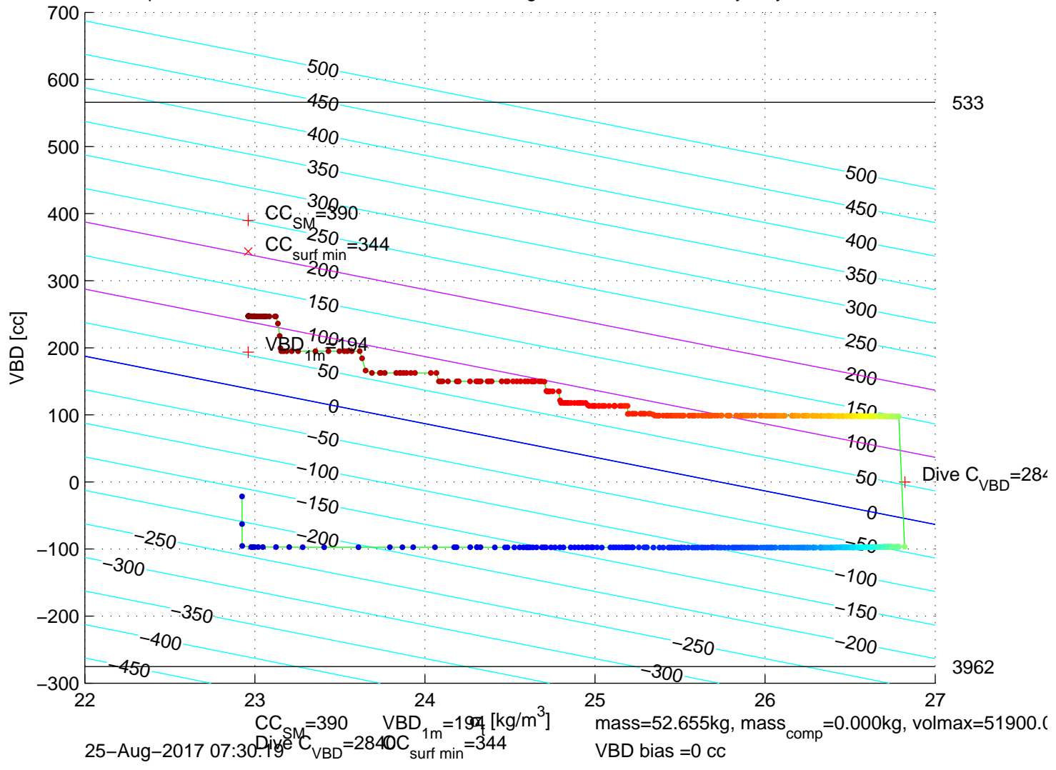
p6350289: SG635 Mission 7 Jul 2017 25-Aug-2017 09:04:19Z – buoyancy contoured
