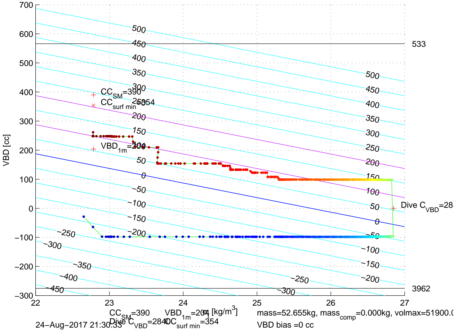
p6350285: SG635 Mission 7 Jul 2017 24-Aug-2017 23:06:02Z – buoyancy contoured
