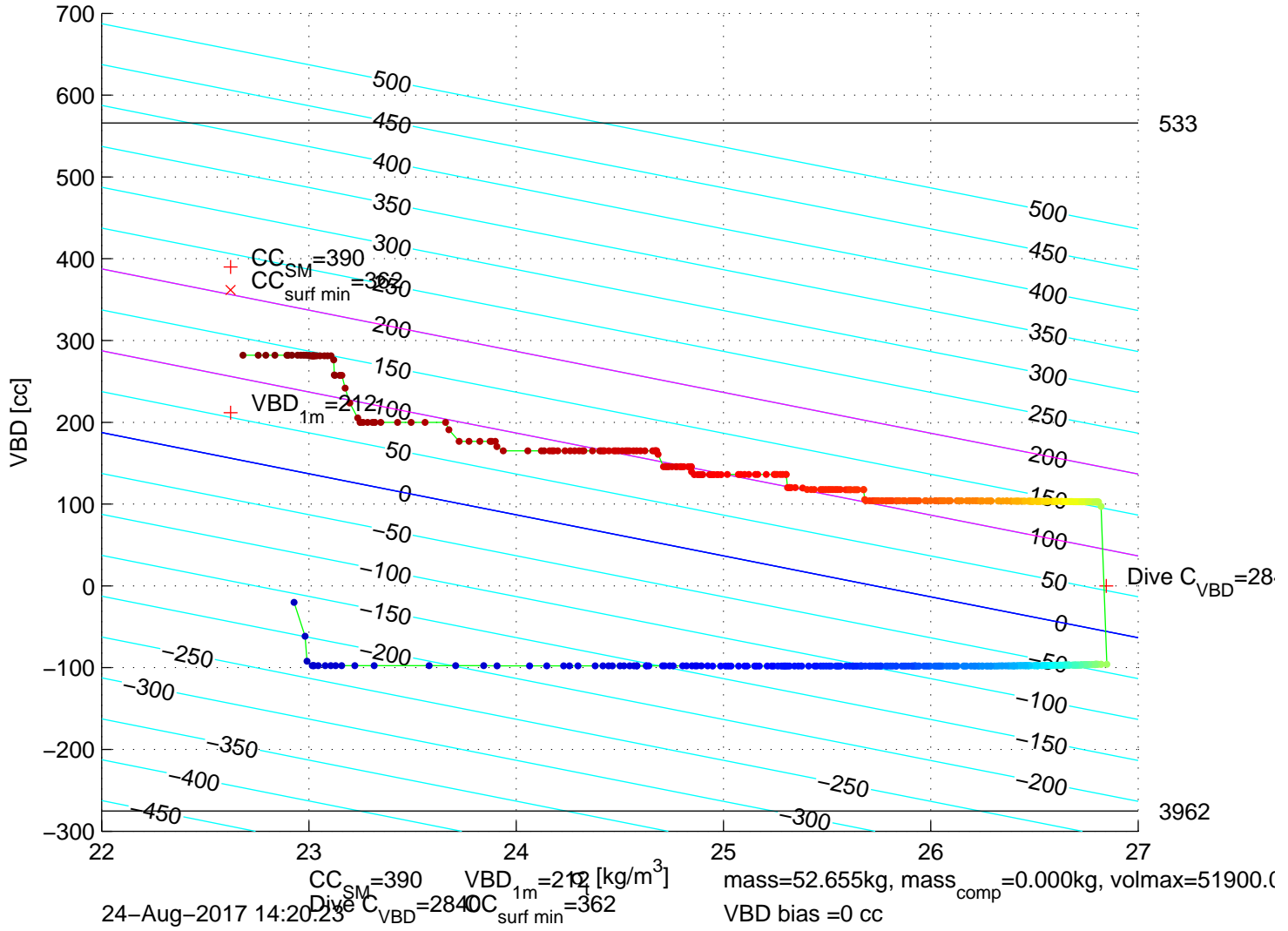
p6350282: SG635 Mission 7 Jul 2017 24-Aug-2017 15:41:20Z – buoyancy contoured
