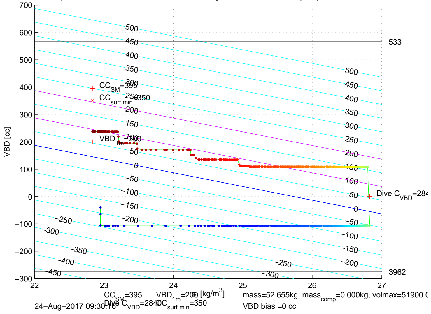
p6350280: SG635 Mission 7 Jul 2017 24-Aug-2017 11:21:33Z – buoyancy contoured
