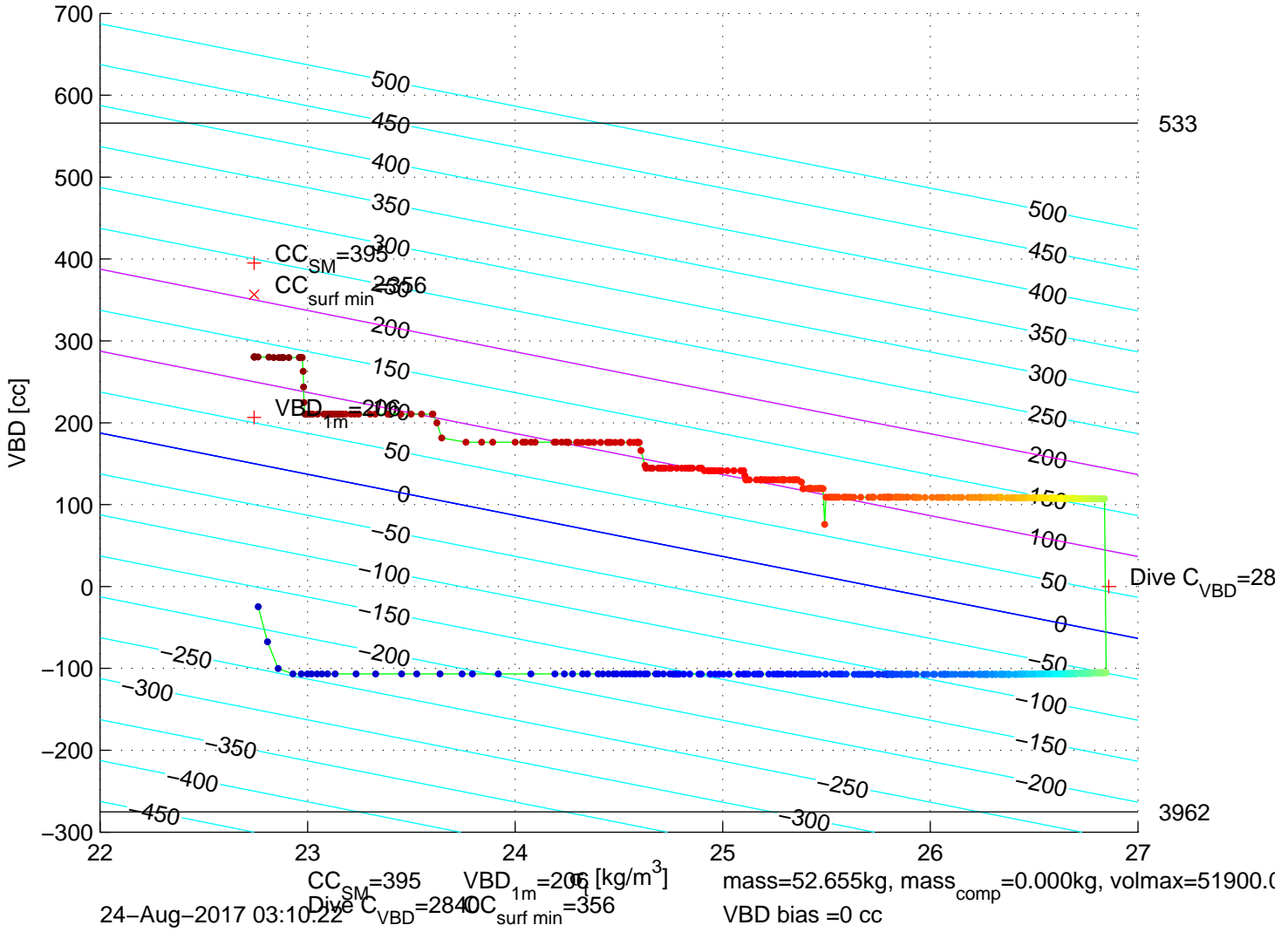
p6350277: SG635 Mission 7 Jul 2017 24-Aug-2017 04:33:43Z – buoyancy contoured
