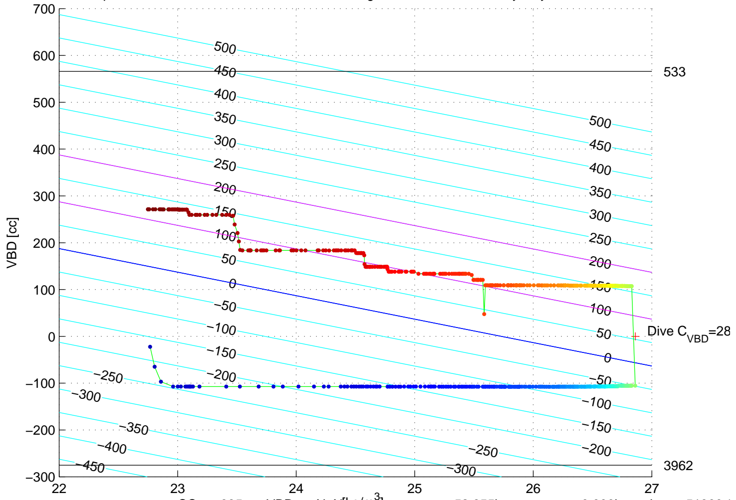
p6350276: SG635 Mission 7 Jul 2017 24-Aug-2017 02:03:34Z – buoyancy contoured
