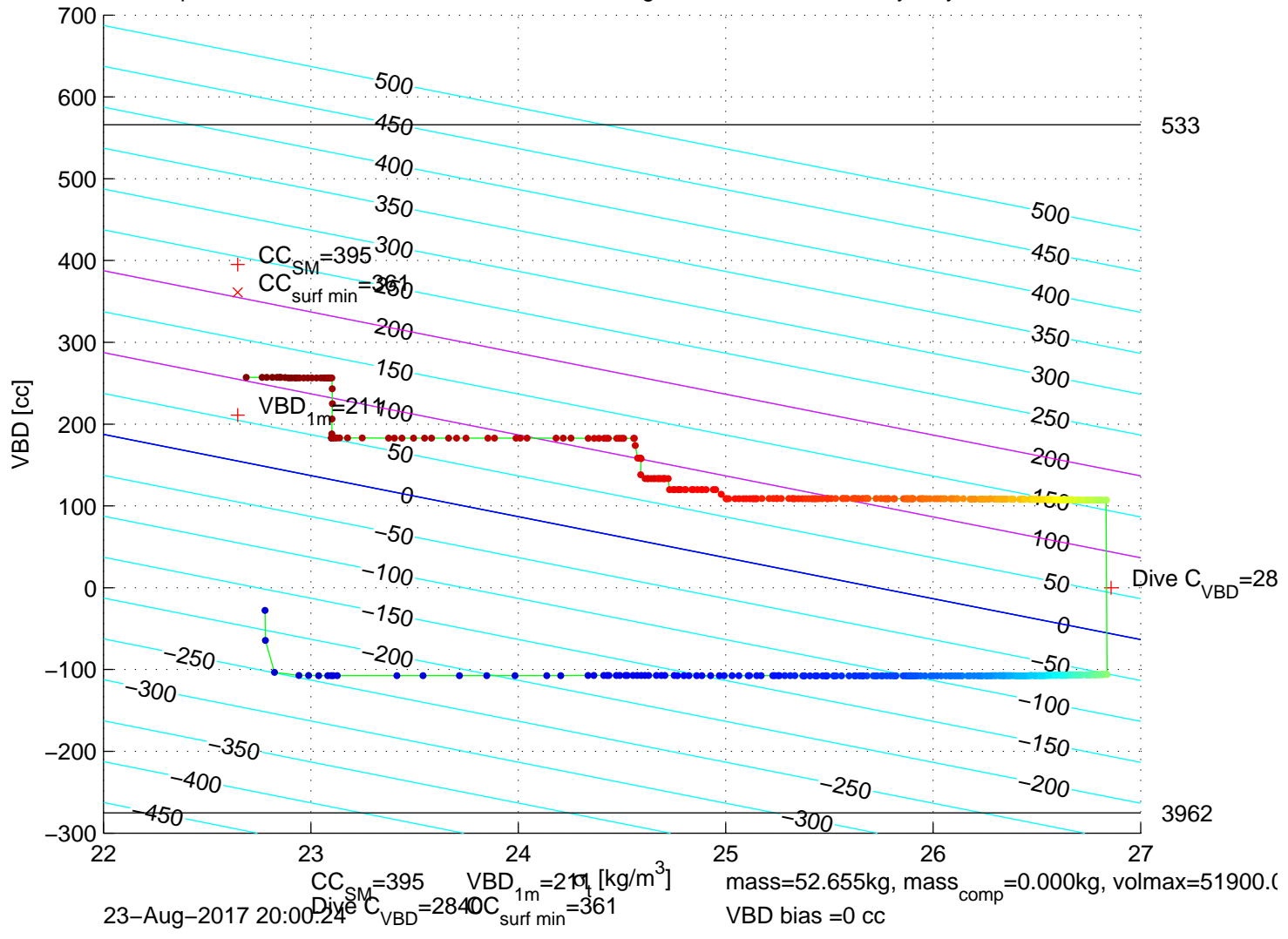
p6350274: SG635 Mission 7 Jul 2017 23-Aug-2017 21:46:43Z – buoyancy contoured
