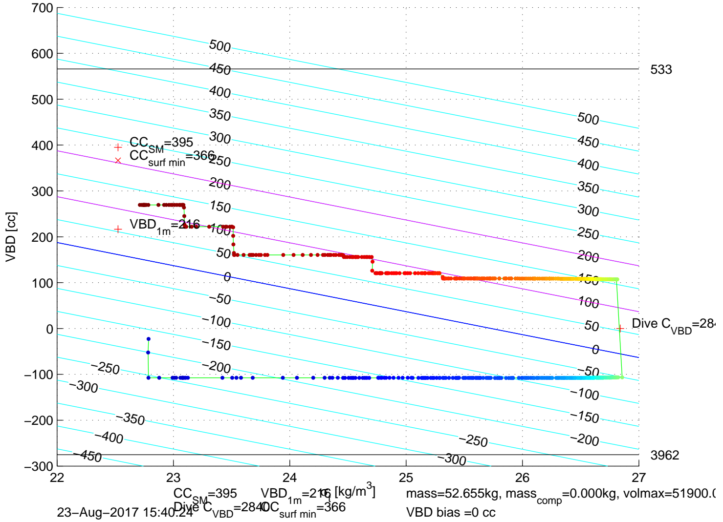
p6350272: SG635 Mission 7 Jul 2017 23-Aug-2017 17:16:33Z – buoyancy contoured
