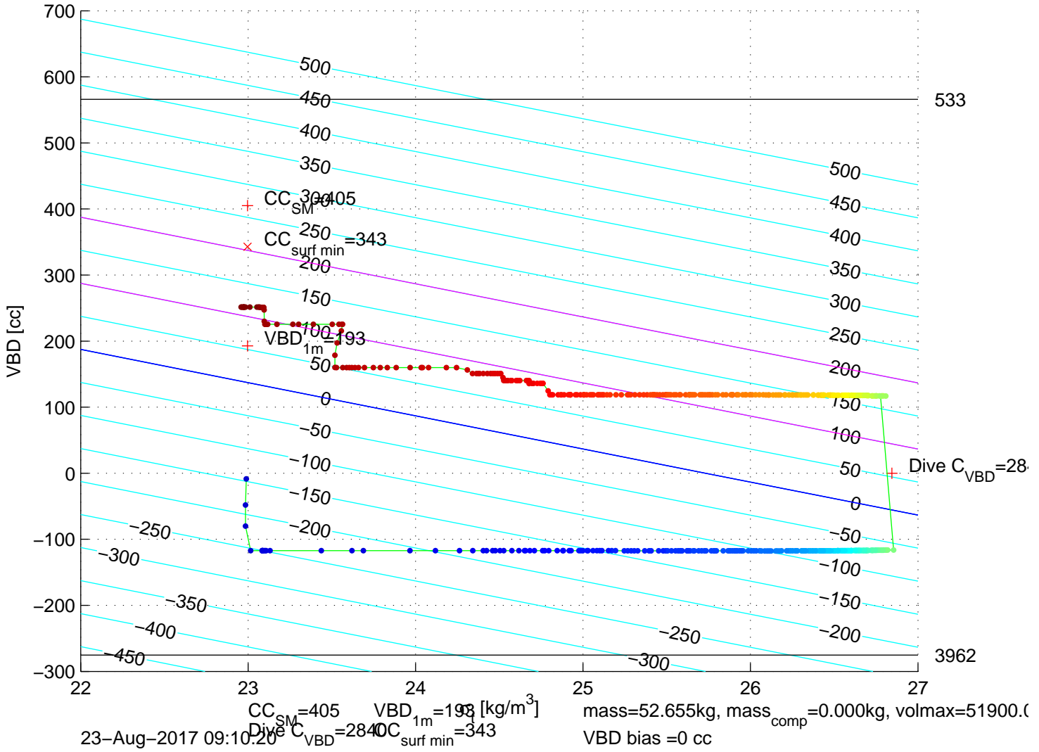
p6350269: SG635 Mission 7 Jul 2017 23-Aug-2017 11:04:39Z – buoyancy contoured
