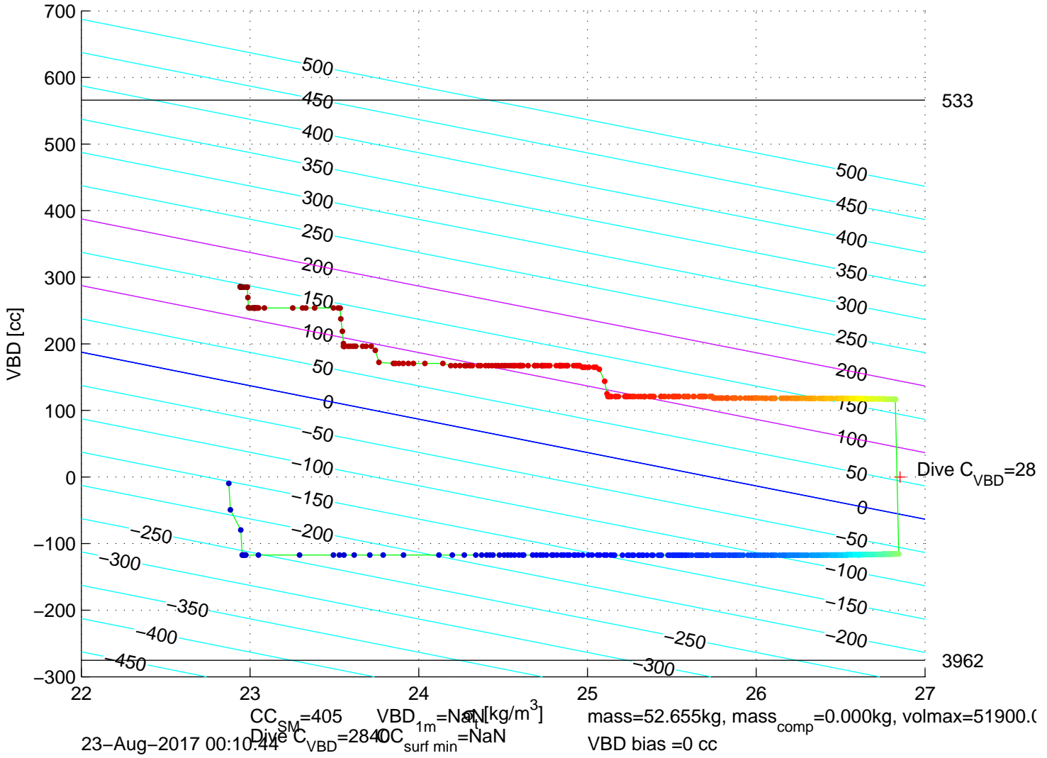
p6350265: SG635 Mission 7 Jul 2017 23-Aug-2017 01:42:56Z – buoyancy contoured
