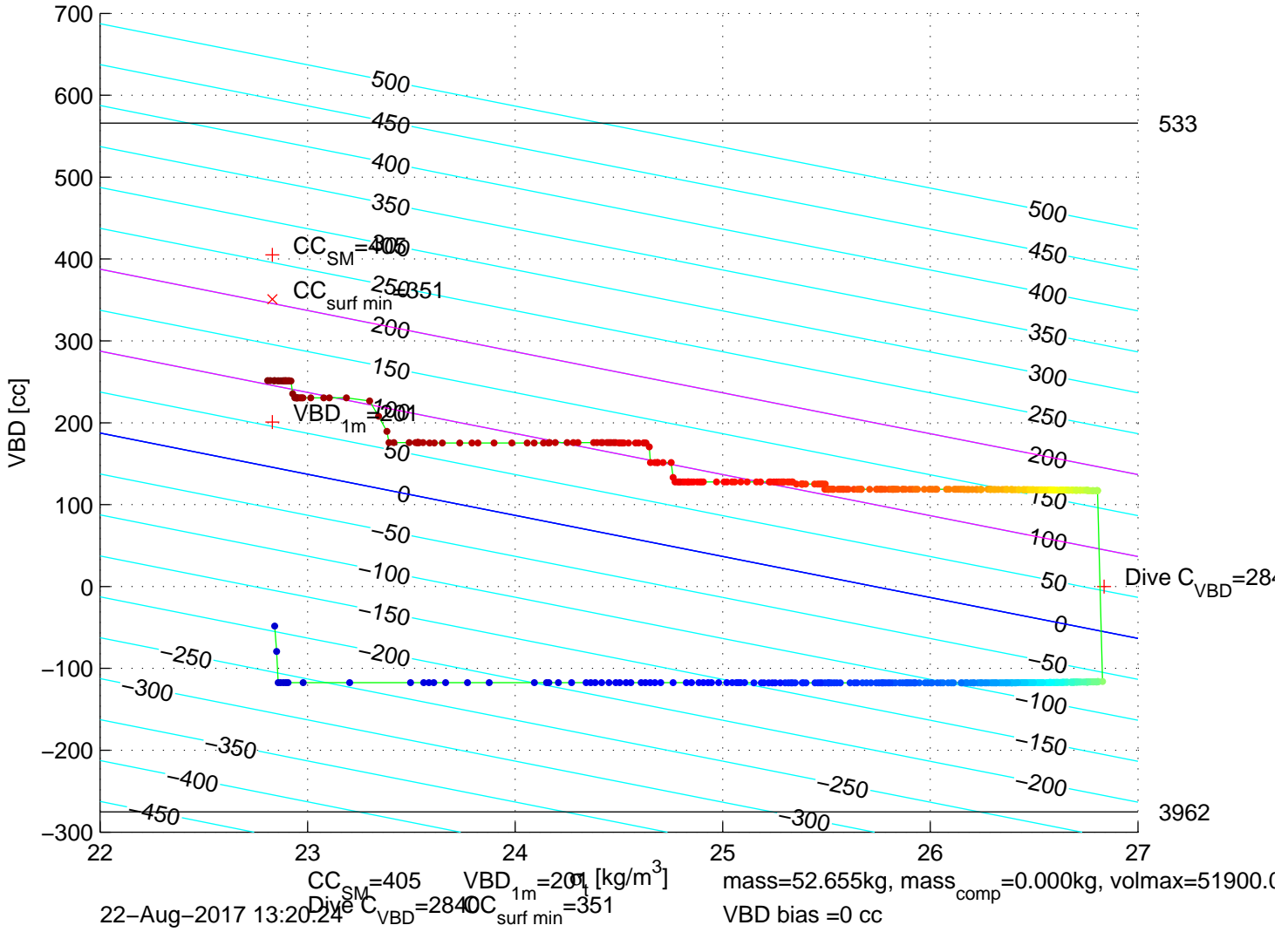
p6350260: SG635 Mission 7 Jul 2017 22-Aug-2017 15:07:54Z – buoyancy contoured
