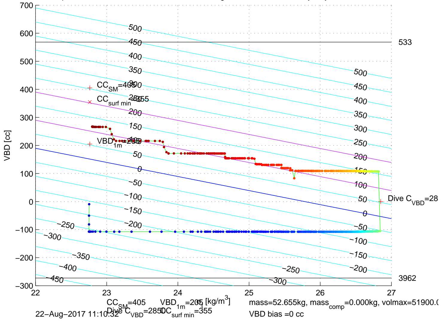
p6350256: SG635 Mission 7 Jul 2017 22-Aug-2017 05:47:19Z – buoyancy contoured
