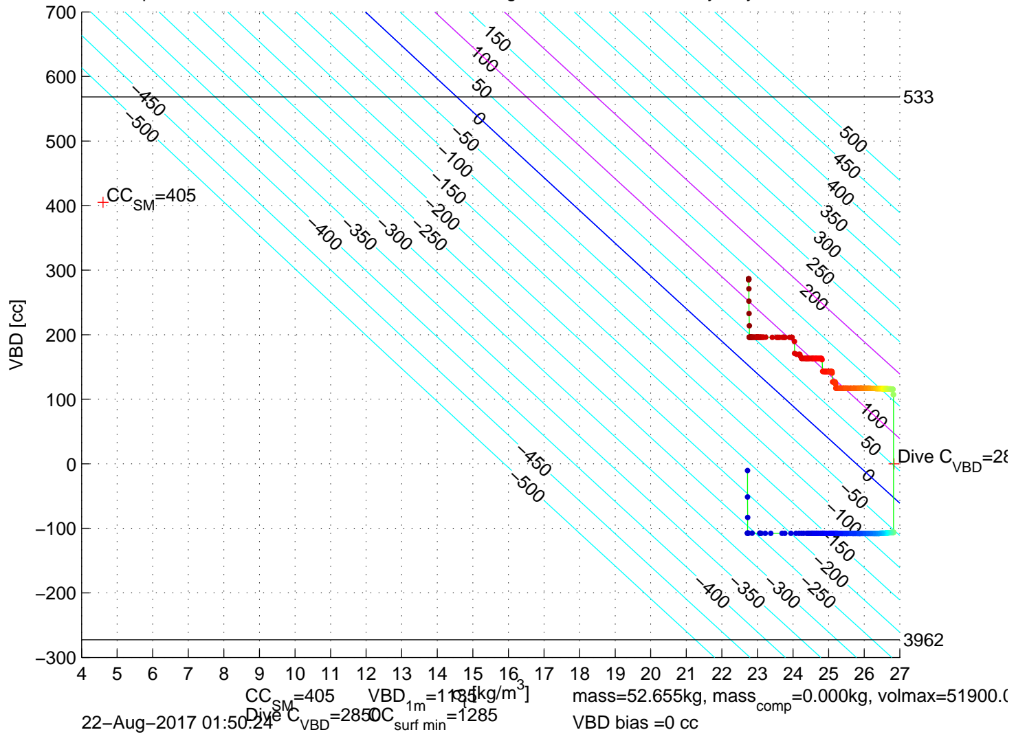
p6350255: SG635 Mission 7 Jul 2017 22–Aug–2017 03:16:32Z – buoyancy contoured
