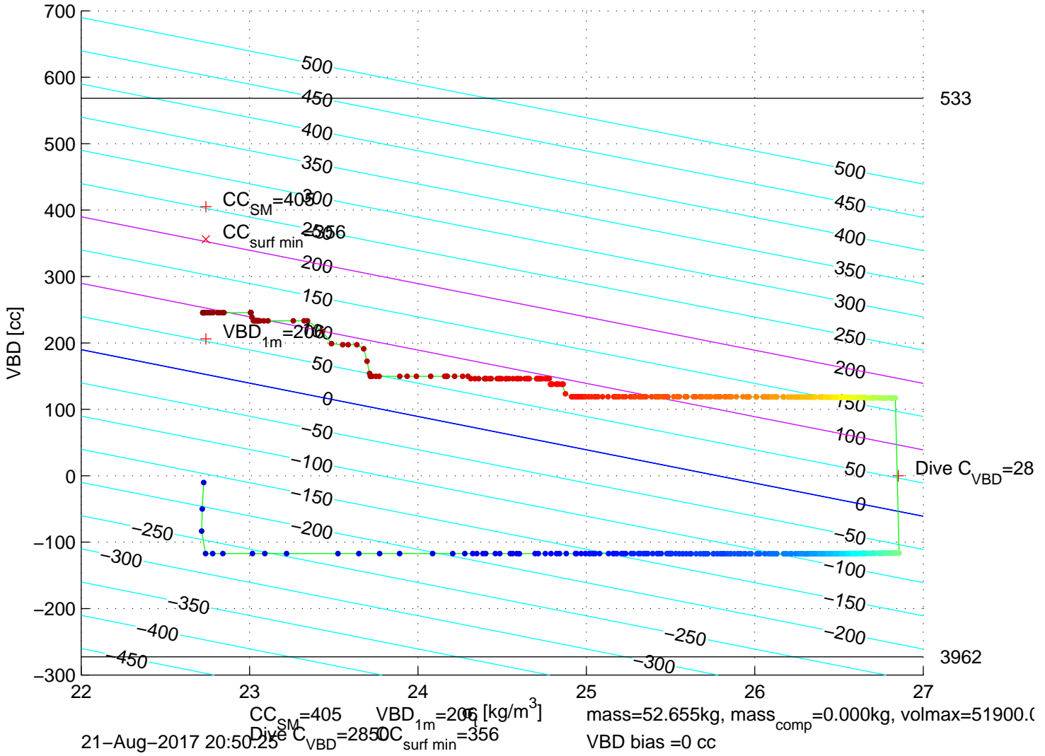
p6350253: SG635 Mission 7 Jul 2017 21-Aug-2017 22:42:36Z – buoyancy contoured
