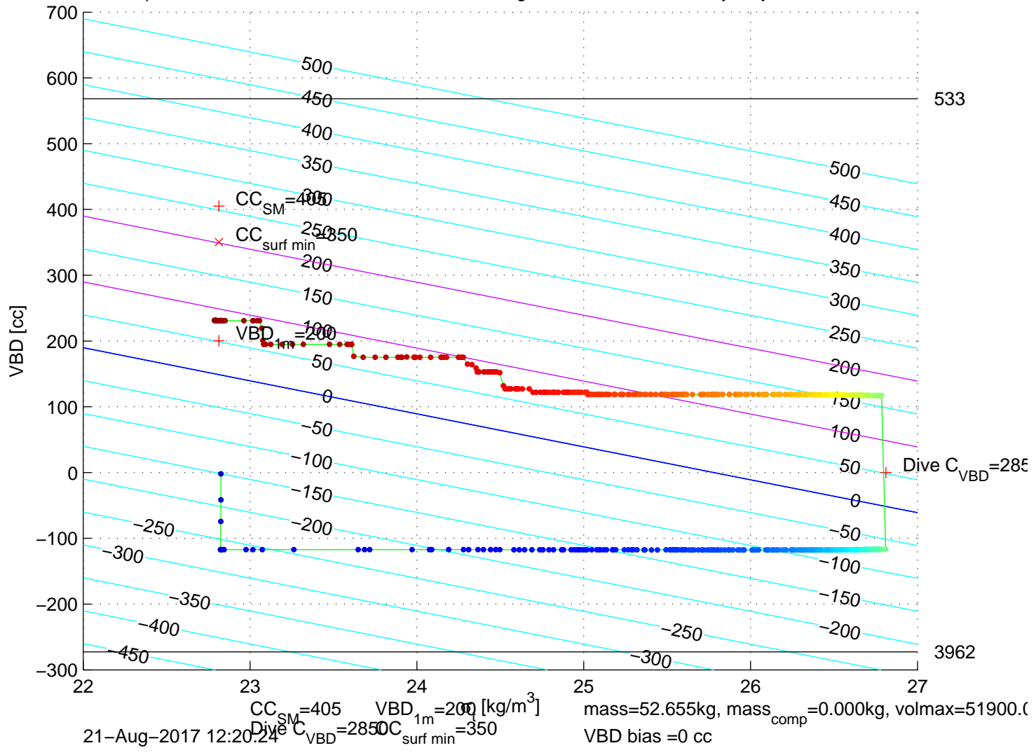
p6350249: SG635 Mission 7 Jul 2017 21-Aug-2017 14:10:22Z – buoyancy contoured
