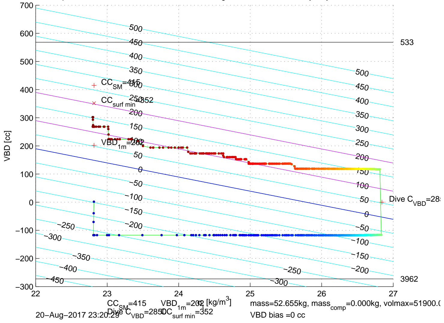
p6350243: SG635 Mission 7 Jul 2017 21–Aug–2017 00:56:24Z – buoyancy contoured
