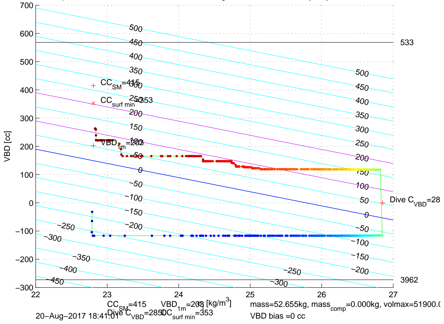
p6350241: SG635 Mission 7 Jul 2017 20-Aug-2017 20:25:57Z – buoyancy contoured
