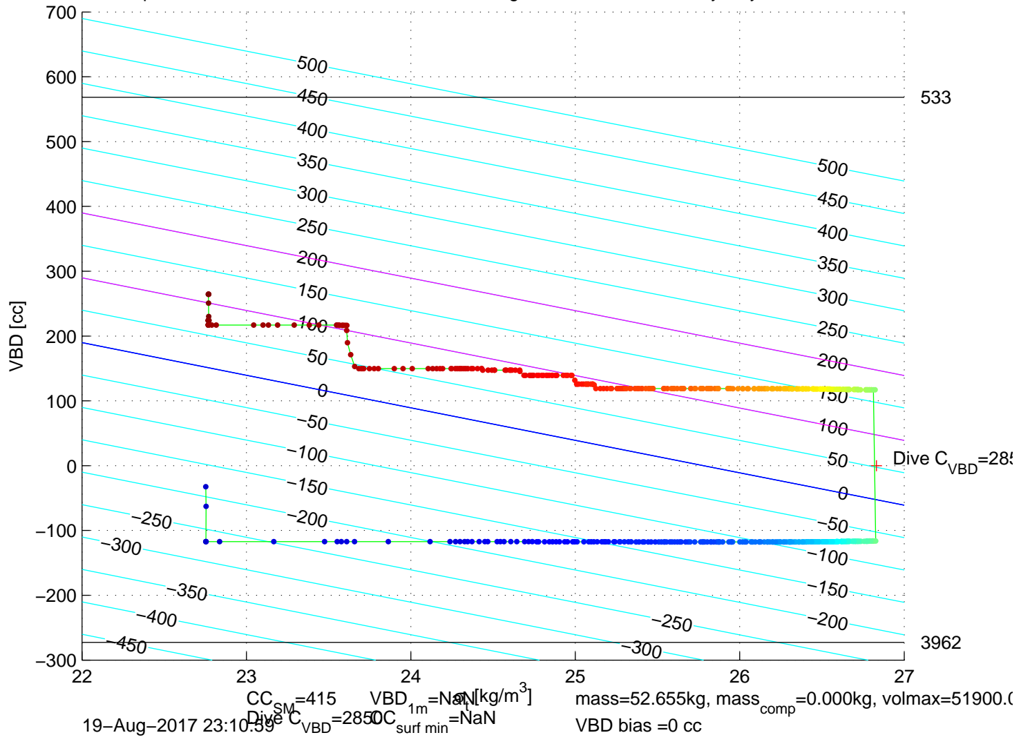
p6350232: SG635 Mission 7 Jul 2017 20-Aug-2017 00:57:38Z – buoyancy contoured
