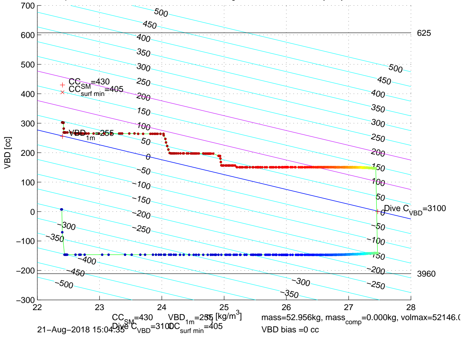
p6350229: SG635 Mission 8 Jul 2018 19-Aug-2018 21:10:11Z - buoyancy contoured
