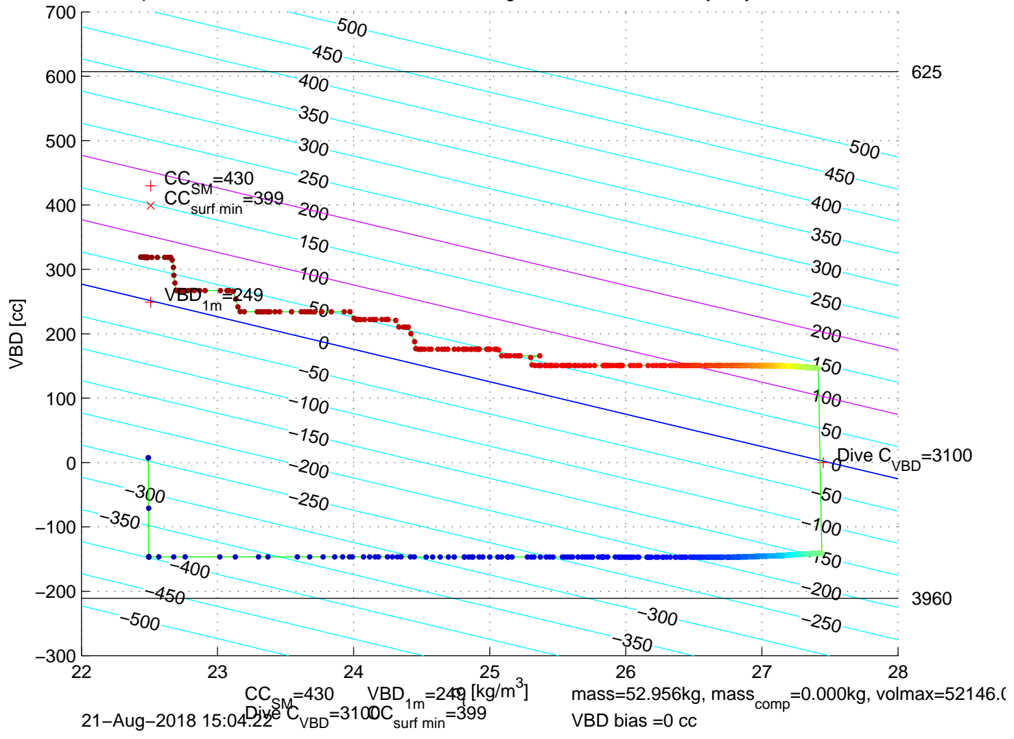
p6350227: SG635 Mission 8 Jul 2018 19-Aug-2018 13:42:43Z – buoyancy contoured
