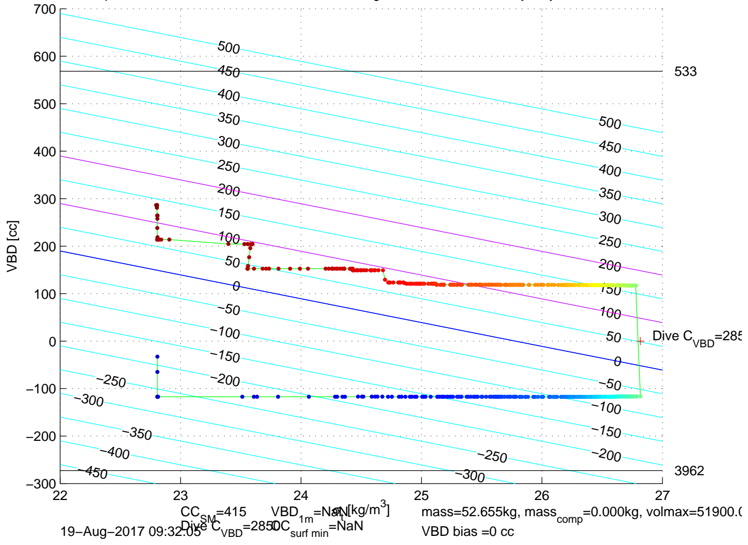
p6350226: SG635 Mission 7 Jul 2017 19-Aug-2017 11:23:12Z – buoyancy contoured
