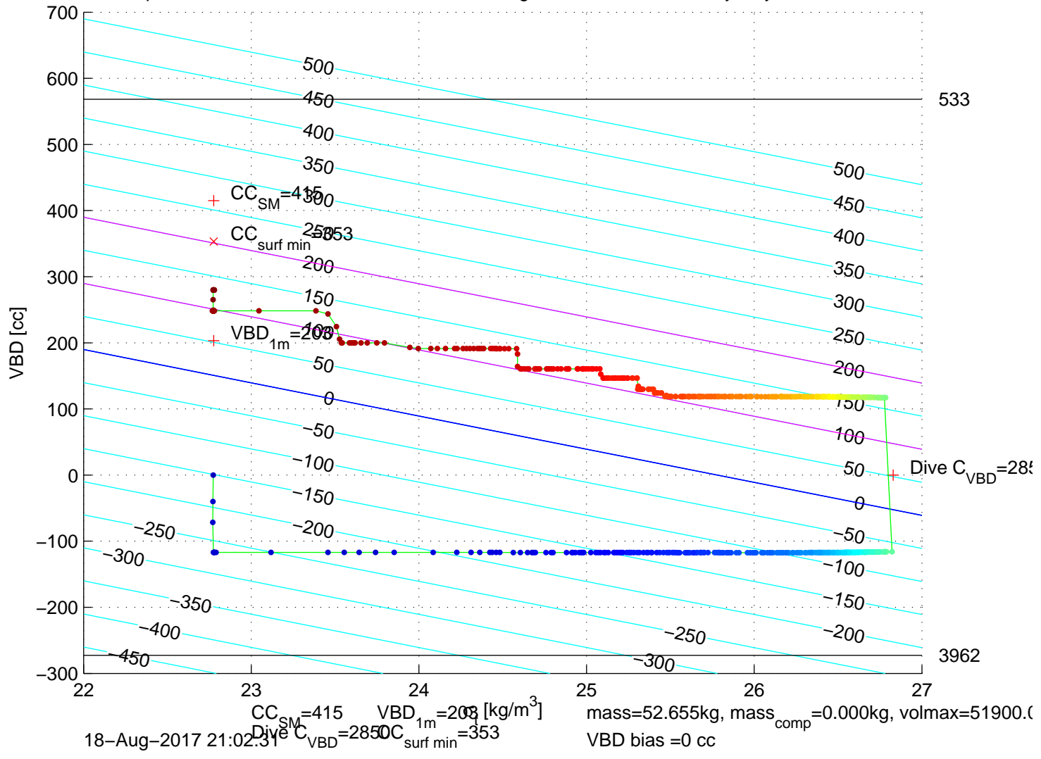
p6350220: SG635 Mission 7 Jul 2017 18-Aug-2017 22:30:28Z – buoyancy contoured
