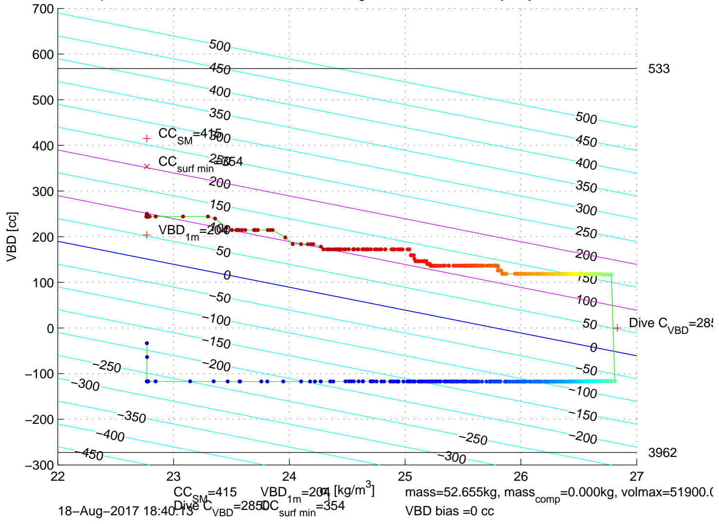
p6350219: SG635 Mission 7 Jul 2017 18-Aug-2017 20:10:42Z – buoyancy contoured
